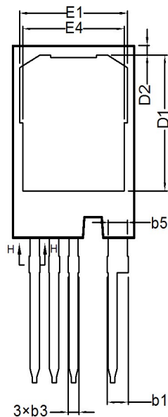
Bottom View
