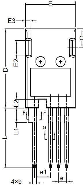
Top View
