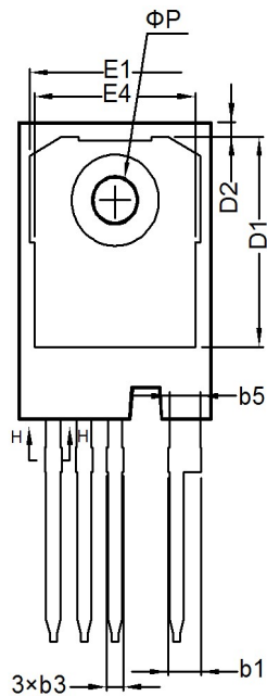
Bottom View
