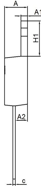
Side View
