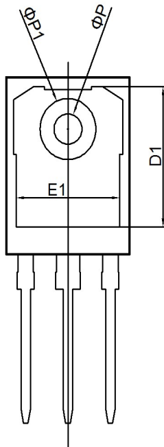
Bottom View
