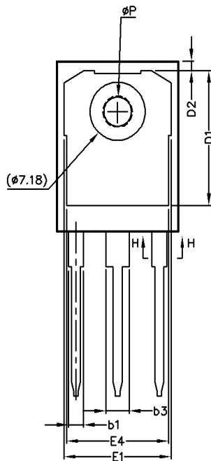
Bottom View
