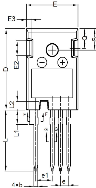
Top View
