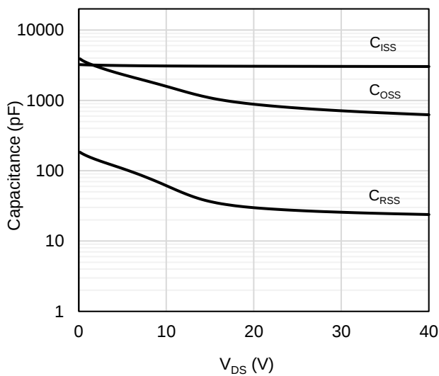
Figure 9: Capacitance Characteristics
