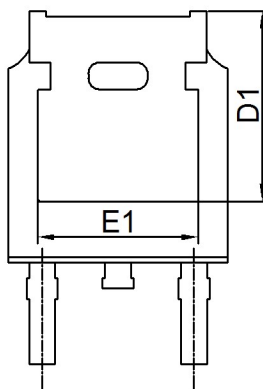
Bottom View
